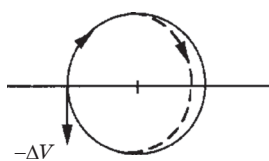
Draw. 2. Formation of the elliptical orbit decreasing velocity of spacecraft flying in a circular (reference) orbit
